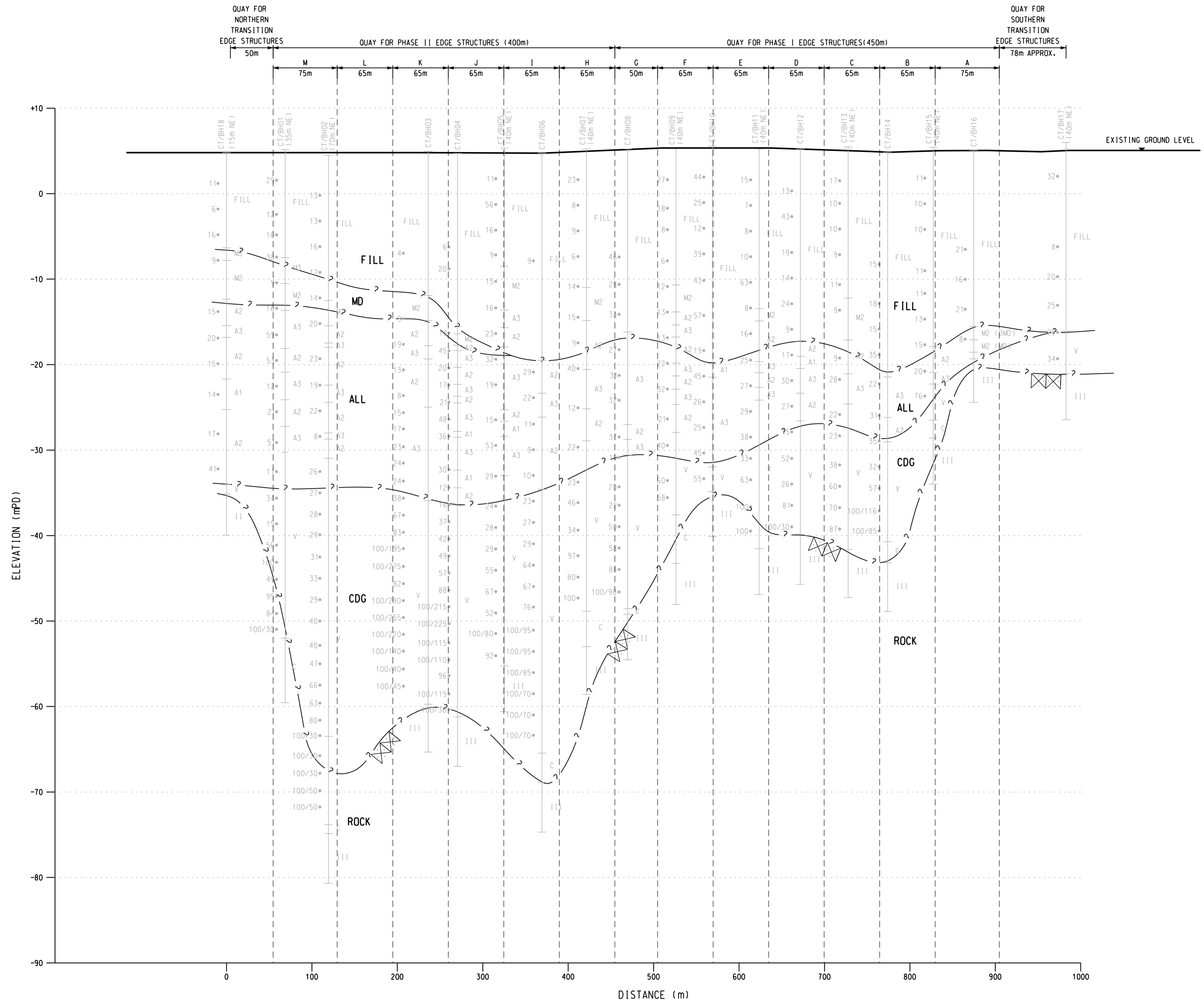
SECTION 1-1 VERTICAL SCALE 1 : 250 HORIZONTAL SCALE 1 : 2500
